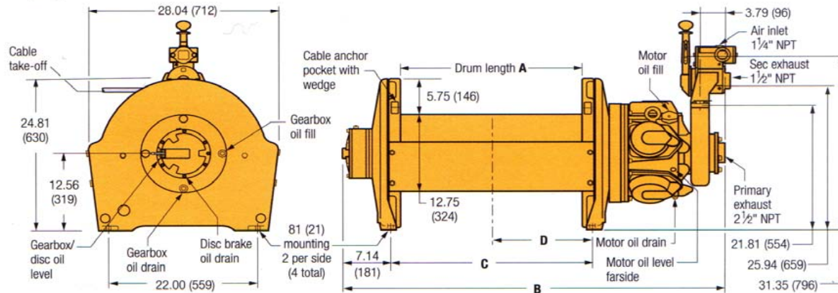
FA5A in inches (mm)
